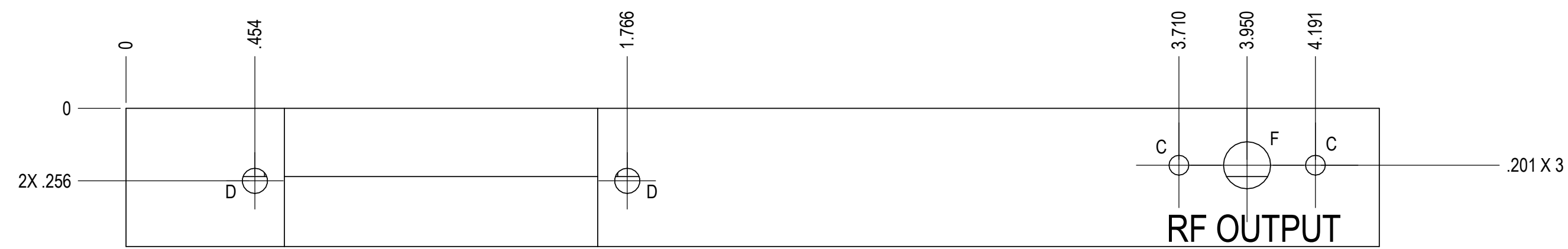
FRONT VIEW
