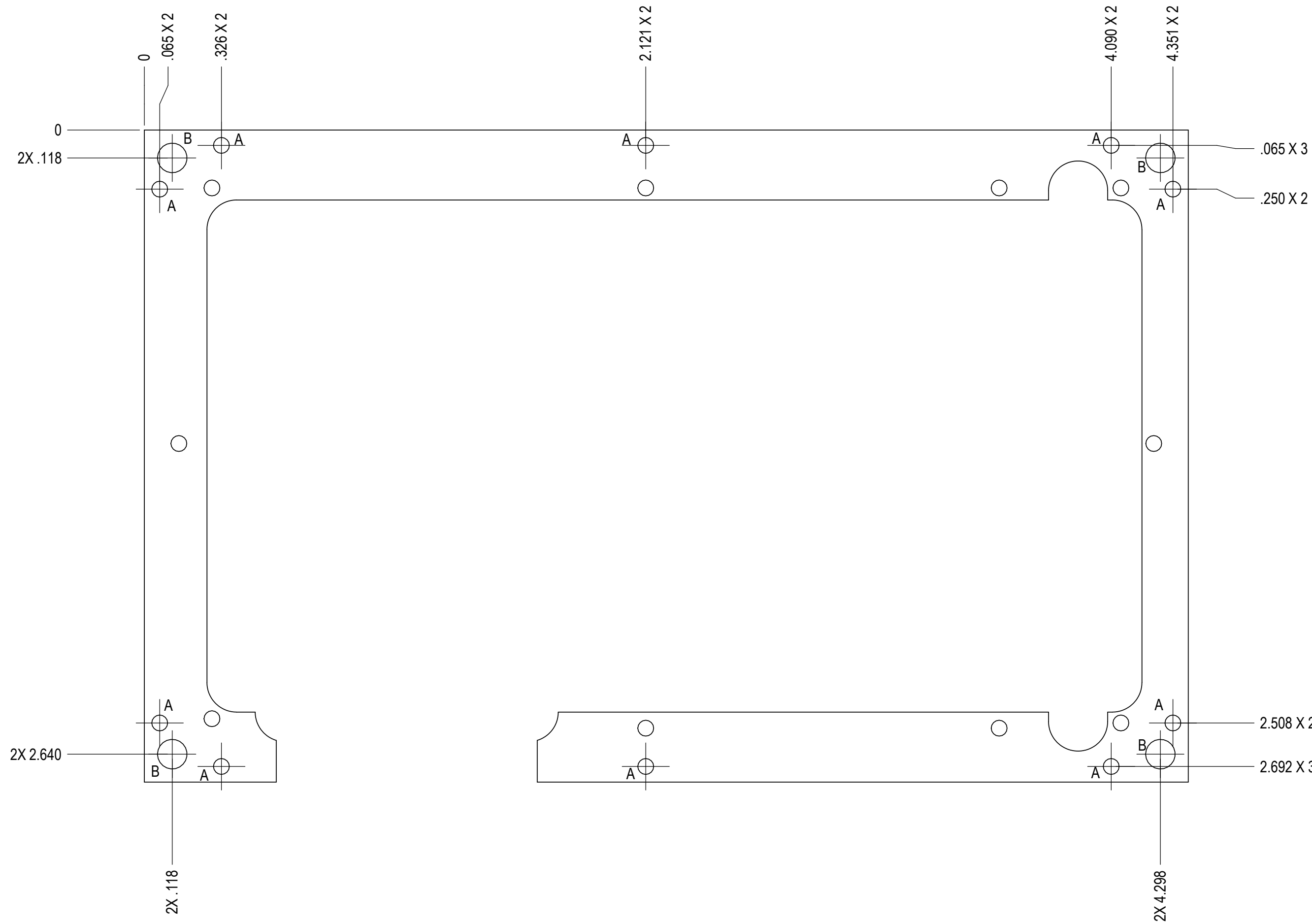
TOP VIEW
